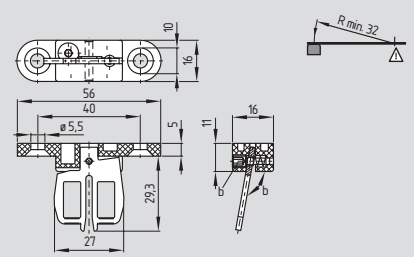
Flexible actuator AZ 15/16-B3
