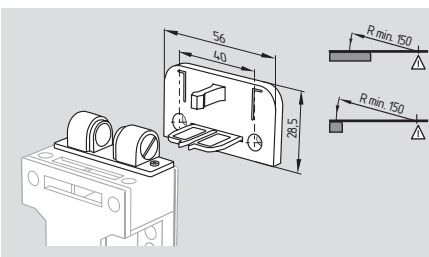
AZ 15/16-B1-2053 with ball latch
