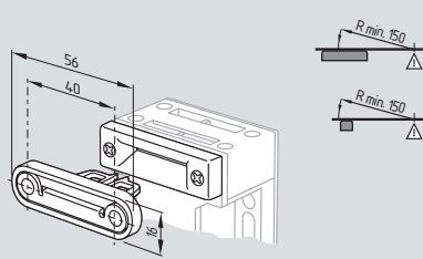
AZ 15/16-B1-2177 with centering guide
